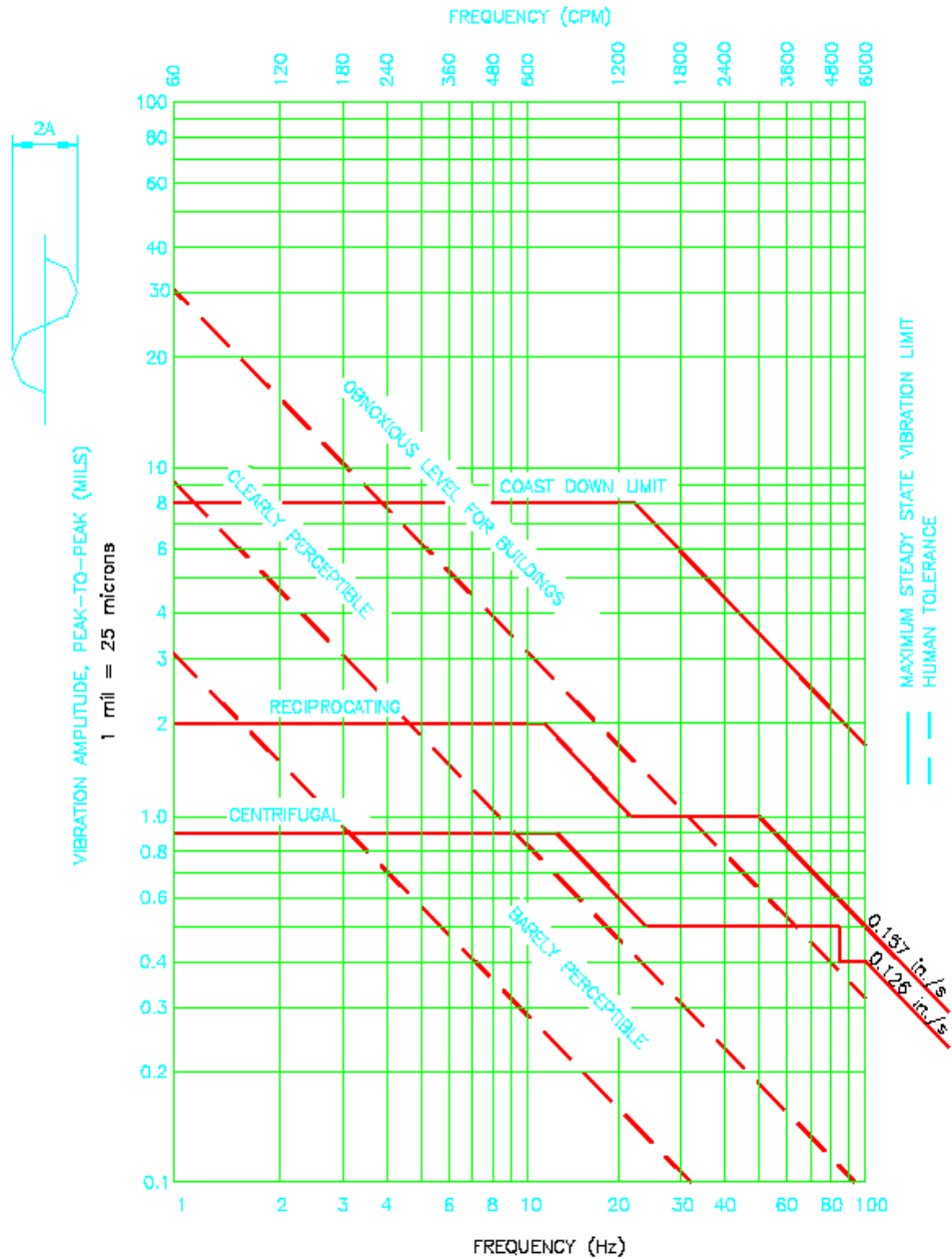
Vibration Limits (21,38)
